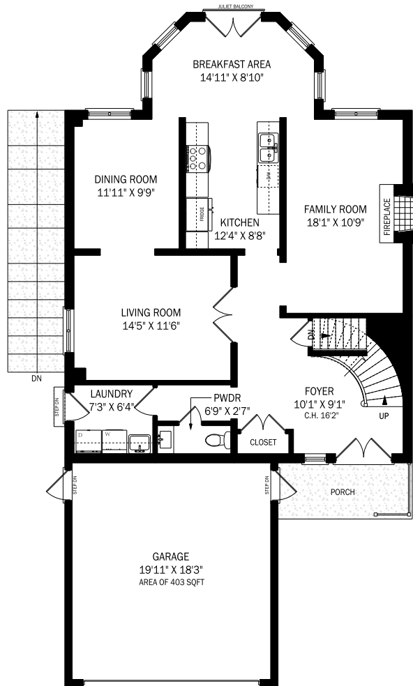
CEILING HEIGHT 8'0" MAIN FLOOR - 1168 SQUARE FEET
